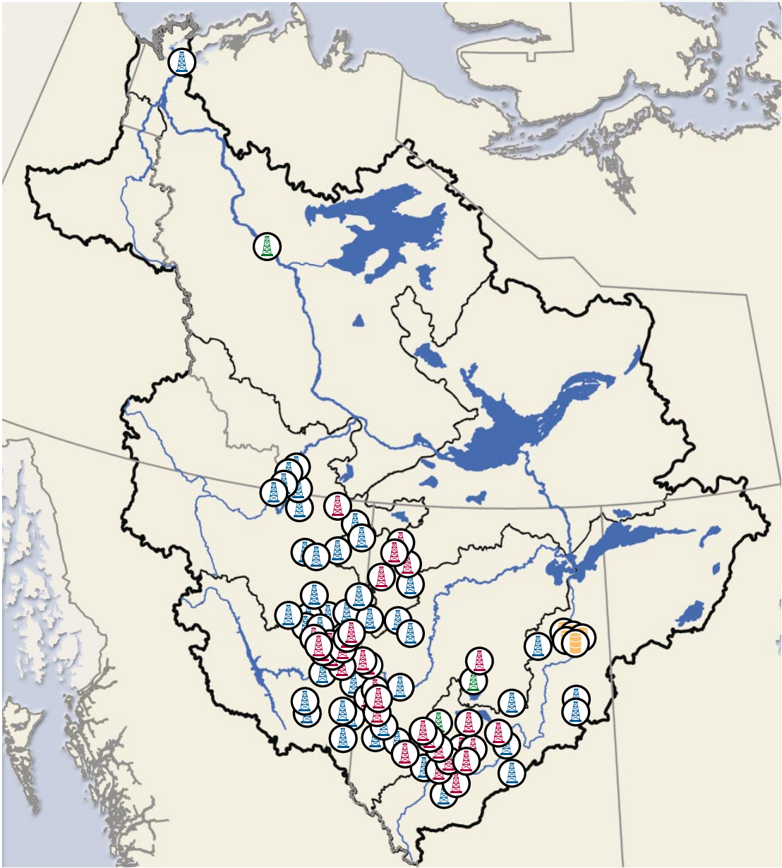
Figure 1–4. Oil and gas fields and oil sands developments in the Mackenzie River Basin. Data Source: Geological Survey of Canada.
