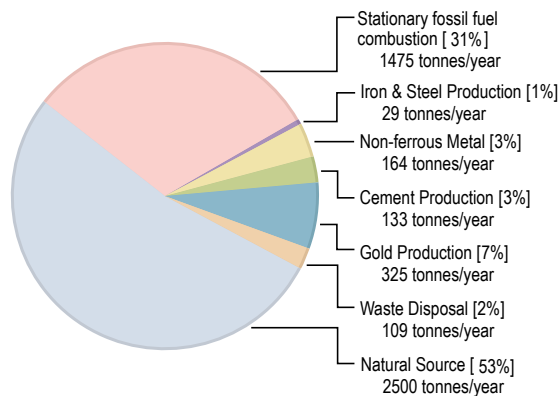
Figure 1–23. Natural and anthropogenic emissions of mercury to the atmosphere
