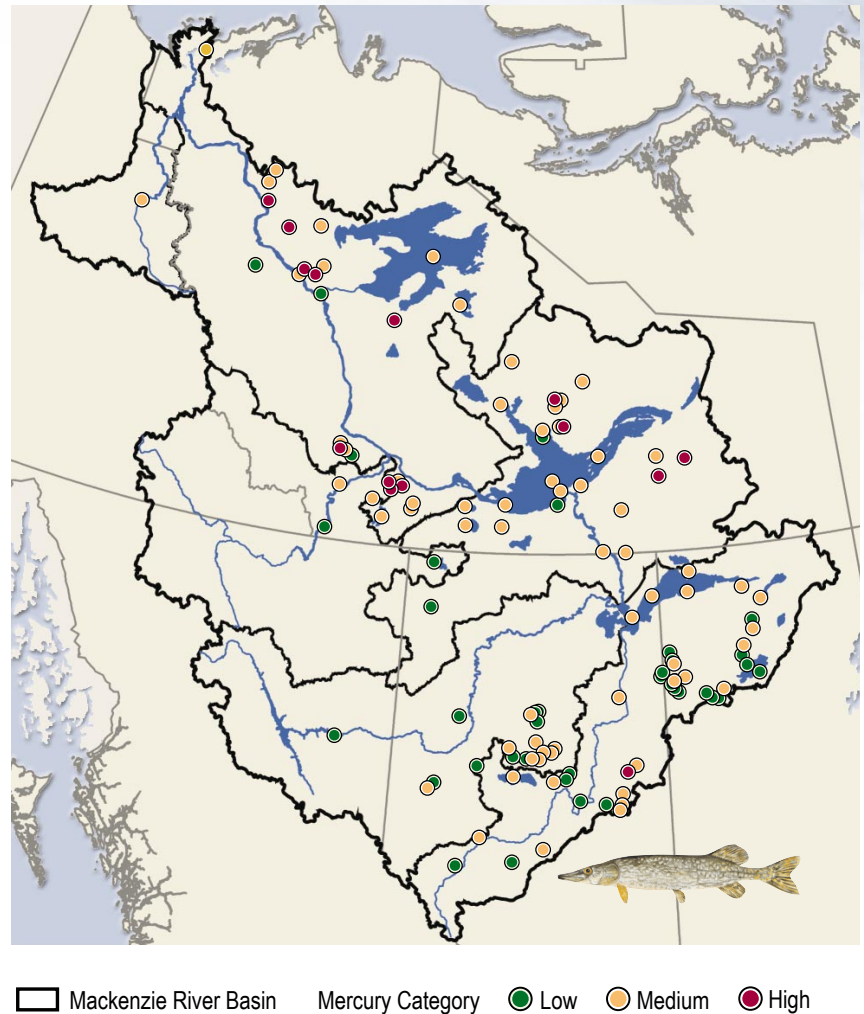
Figure 1–19. Mercury in northern pike at different locations in the Mackenzie River Basin.
